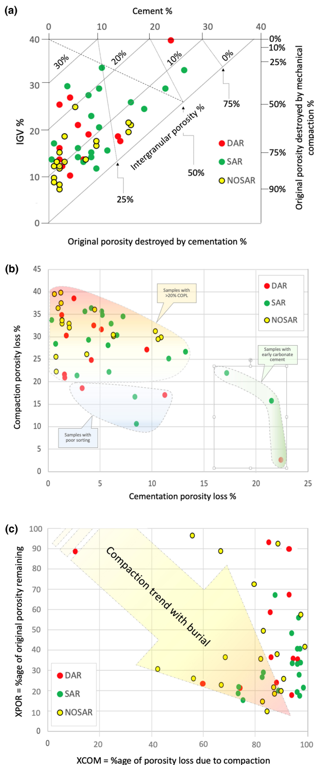
FIGURE 12 (a) Percentage IG% plotted against intergranular cement determined from thin section modal analysis using the Ehrenberg (1989) modification of the Housenecht (1987) calculations. Most samples have low IG% with most original porosity being destroyed by mechanical compaction. Three samples with >30% IG% contain early carbonate cements. (b) Graph of percentage compactional porosity loss (COPL) and porosity loss by cementation (CEPL) in the Ghaggar-Hakra Formation sandstones highlighting the main groupings. Except for sandstones with early carbonate cements, most porosity loss is from mechanical compaction. COPL and CEPL calculations from Ehrenberg (1995). (c) Graph of percentage of porosity loss due to compaction (XCOM) against the percentage of original porosity remaining (XPOR). The data indicates that the Ghaggar-Hakra sandstones record the end product of extensive mechanical compaction, consistent with the COPL vs CEPL plot, most likely the result of rapid burial in the Paleocene. Sandstones retaining a high percentage of original porosity contain early carbonate cements. Calculations of XCOM and XPOR from Ehrenberg (1995). Legend on all graphs: DAR—Darjaniyon-ki Dhani Sandstone; SAR—Sarnoo Sandstone and NOSAR—Nosar Sandstone.
